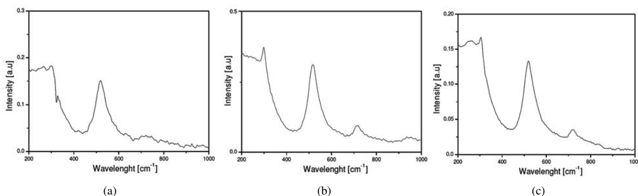
Figure 3. Raman spectra of \text{Y}_3\text{Fe}_{5-x}\text{Al}_x\text{O}_{12} powders synthesized at 700^\circ\text{C} for 2 h by the polymeric precursor method with: a) x = 1.5 , b) x = 1.6 and c) x = 1.7
