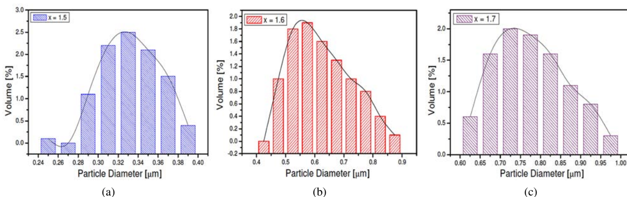
Figure 4. Hydrodynamic particle size distribution of \text{Y}_3\text{Fe}_{5-x}\text{Al}_x\text{O}_{12} with: a) x = 1.5 , b) x = 1.6 and c) x = 1.7
