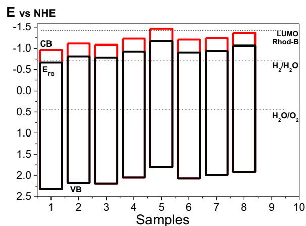
Fig. 11. Band positions of samples in carbon paste electrode in NaOH (1 mol L -1 ) solution. CB: conduction band, VB: valence band, EFB: flat band potential.
