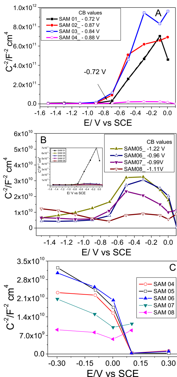
Fig. 10. Mott-Schottky plots of ZnO:N samples at fixed frequency of 159 Hz in the dark and a potential amplitude of 10 mV in NaOH (1 mol L -1 ) solution. CB values = conduction band values obtain from Mott-Schottky plots vs SCE.
