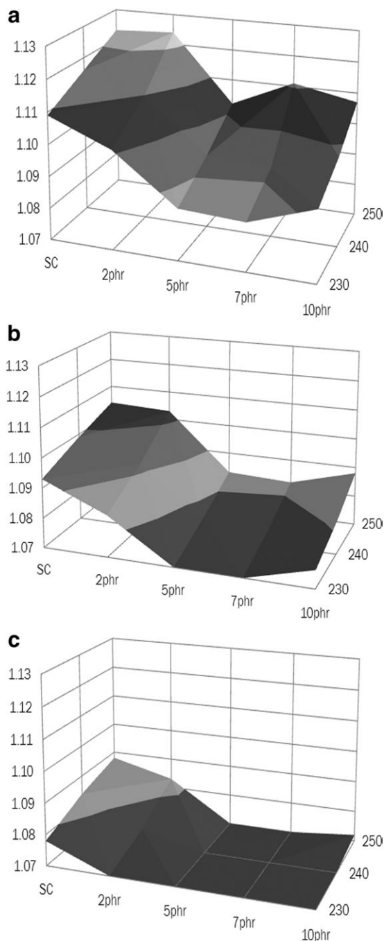
Figure 3. Specific volume variations with temperature and pressures ( x axis—compatibilizer content [phr]; y axis—temperature [ ^{\circ}\text{C} ]; z axis—specific volume [ \text{cm}^3/\text{g} ]), being the gray gradient relative to different specific volume ranges. Pressures: (a) 20 MPa, (b) 40 MPa, and (c) 60 MPa.
