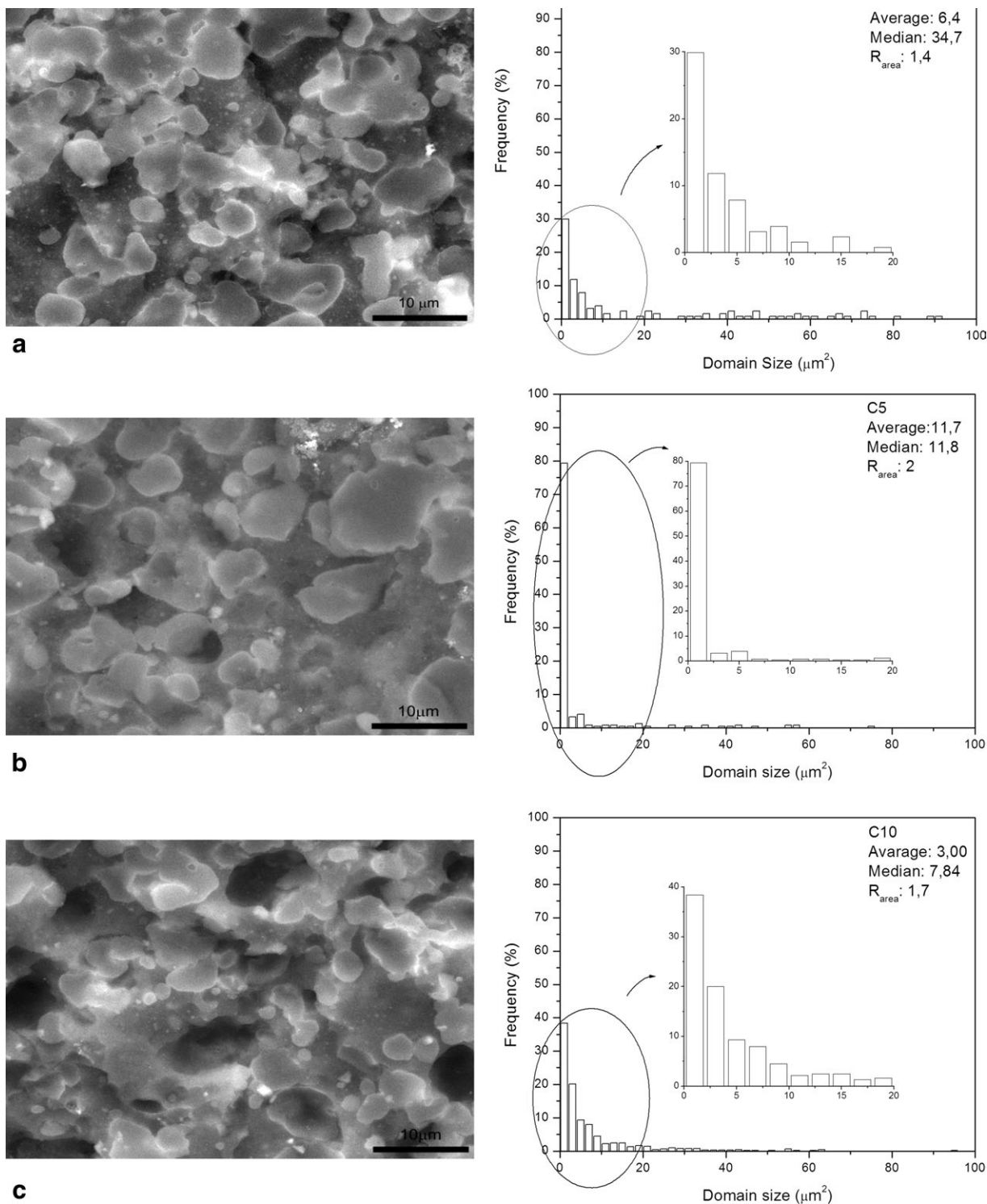
Figure 5. SEM images and domain size distribution of (a) Czero, (b) C5, and (c) C10 samples, where the brighter areas are the \text{OsO}_4 stained NBR phase, and the distribution step in all graphics correspond to 2 \mu\text{m}^2 of diameter.
