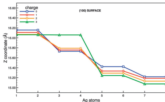
Fig. 8 Z coordinates of the surface Ag atoms for each charge addition.
