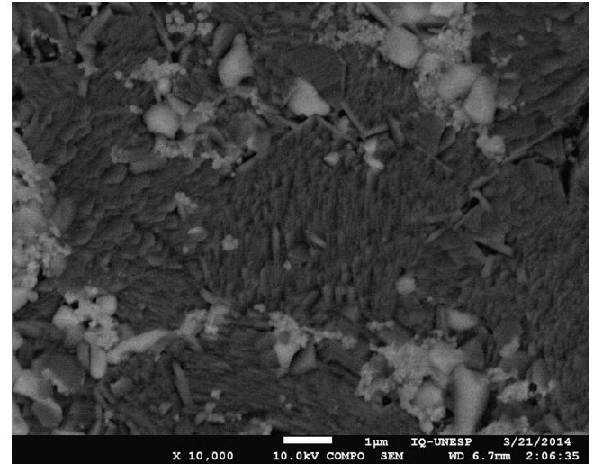
Fig. 9. FEG microstructure of NZF(70–30)–BT composite sintered at 1200\text{ }^\circ\text{C} for 2 h.
