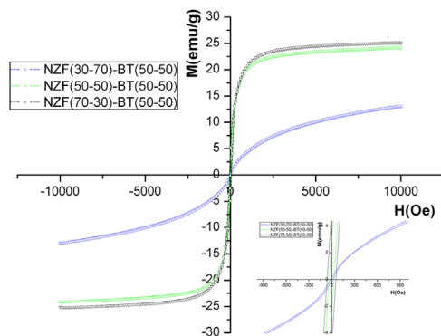
Fig. 14. Magnetic hysteresis loops at room temperature for all composite ceramics.
