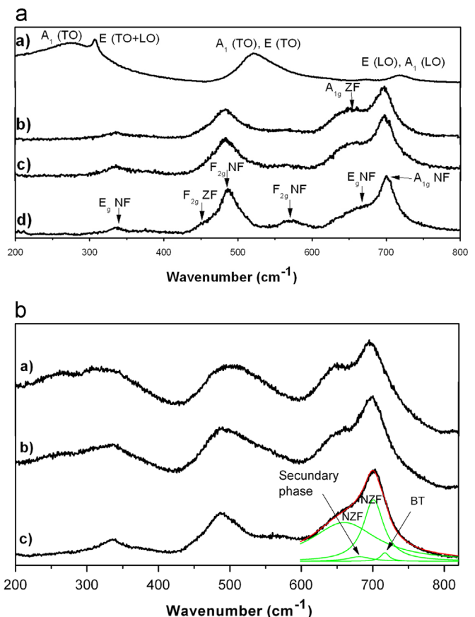
Fig. 7. (a) Raman spectra of (a) BT, (b) NZF(30–70), (c) NZF(50–50), and (d) NZF(70–30) and (b) Raman spectra of composites (a) NZF(30–70)–BT, (b) NZF(50–50)–BT and (c) NZF(70–30) at room temperature.
