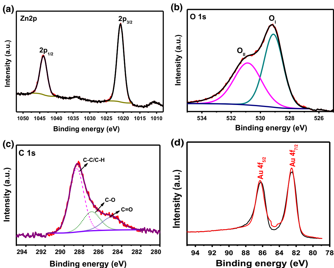
Fig. 3 XPS spectra of (a) Zn 2p XPS spectrum; (b) O1s XPS spectrum; (c) C1s XPS spectrum of pure ZnO NRs, and (d) Au 4f for the gold-ZnO NRs
