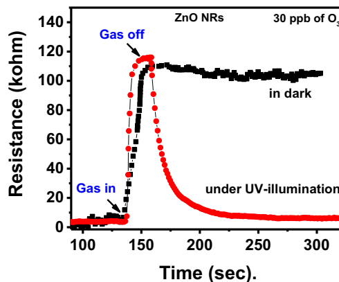
Fig. 4 Resistive response curve of pure ZnO NRs exposed to 30 ppb of O 3 gas under dark and continuous UV irradiation at room temperature
