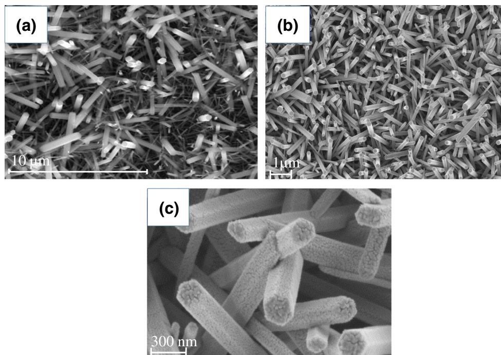
Fig. 2 FESEM images of (a) pure ZnO NRs and (b-c) low and high magnification gold-ZnO NRs
