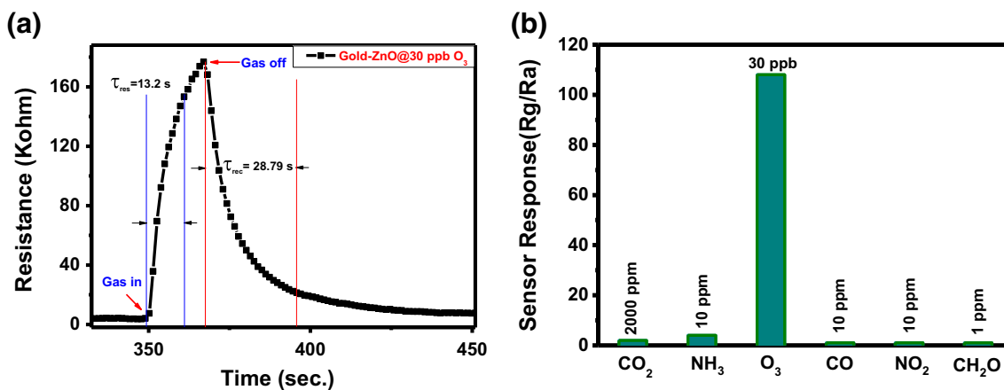
Fig. 6 a Typical response-recovery characteristics of gold-ZnO sensor at room temperature for 30 ppb of ozone with UV activation. b Selectivity histogram of the gold-ZnO sensor to several possible interferents at room temperature under UV-illumination
