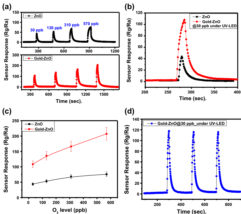
Fig. 5 (a) Room-temperature gas sensing response of ZnO and gold-ZnO for various O 3 gas concentrations under continuous UV-illumination. (b) Comparative plot of sensor responses for pure and gold-ZnO NRs exposed to 30 ppb of O 3 gas. (c) Variation of sensor response as a function of ozone concentration for pure and gold-ZnO NRs. (d) Reproducibility of the three gold-ZnO sensors for 30 ppb of O 3 gas at room temperature with UV illumination
