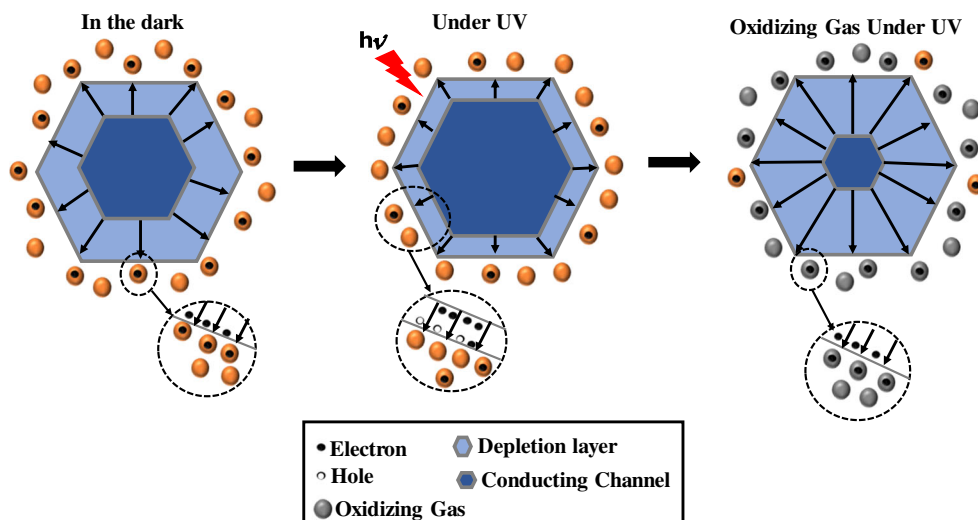
Fig. 7 Schematic illustration of the gas sensing mechanism for the ZnO NRs
