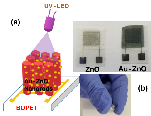
Fig. 1 Schematic illustration: (a) UV-enhanced flexible ZnO sensor; (b) Photos of flexible interdigitated electrodes fabricated with pristine ZnO and gold-ZnO
