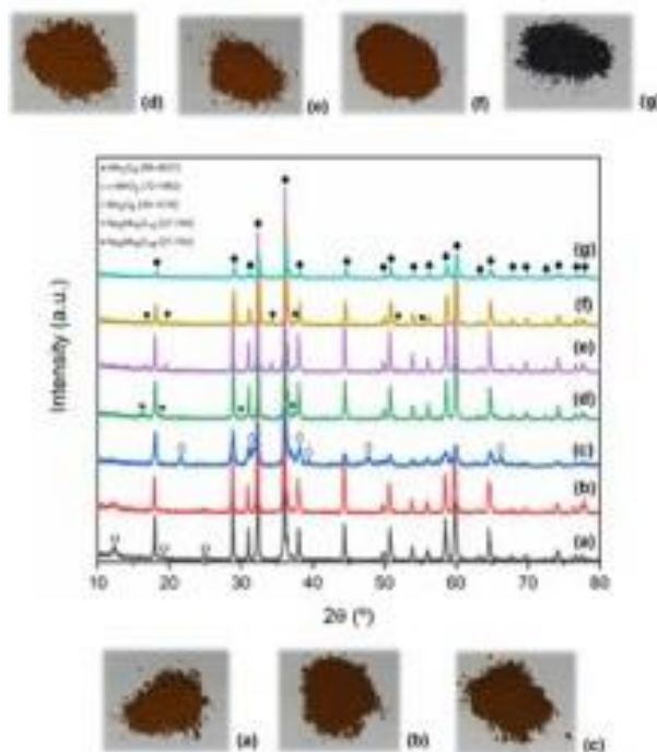
Figure 3: XRD patterns and digital images of the samples (a) MnO, (b) MnO 160 °C, (c) MnO 480 °C, (d) MnO 715 °C, (e) MnO 870 °C, (f) MnO 920 °C e (g) MnO 1150 °C. Assignments: ♦ = tetragonal \text{Mn}_3\text{O}_4 (JCPDS 89-4837), ○ = tetragonal \alpha\text{-MnO}_2 (JCPDS 72-1982), ◇ = monoclinic \text{Mn}_5\text{O}_8 (JCPDS 39-1218), * = monoclinic \text{Na}_2\text{Mn}_5\text{O}_{10} (JCPDS 27-749) and ● = orthorhombic \text{Na}_4\text{Mn}_9\text{O}_{18} (JCPDS 27-750).
