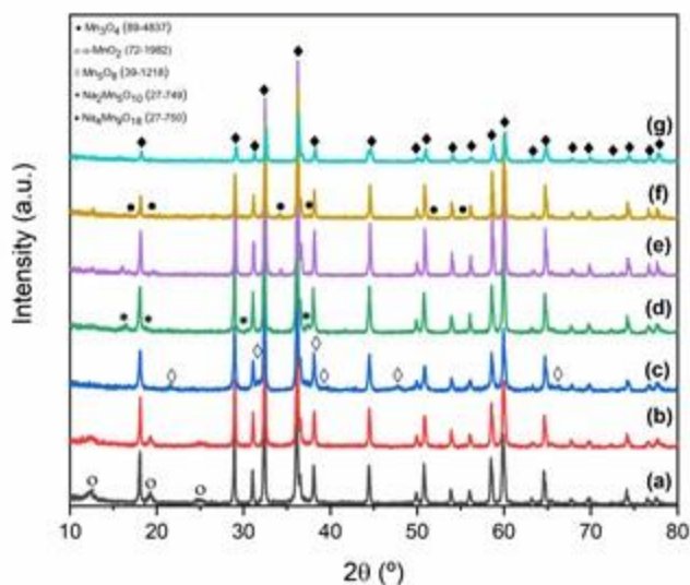
Annex 1: XRD patterns of the replicated samples (a) MnO, (b) MnO 160 °C, (c) MnO 480 °C, (d) MnO 715 °C, (e) MnO 870 °C, (f) MnO 920 °C e (g) MnO 1150 °C. Assignments: \blacklozenge = tetragonal Mn_3O_4 (JCPDS 89-4837), \circ = tetragonal \alpha - MnO_2 (JCPDS 72-1982), \diamond = monoclinic Mn_5O_8 (JCPDS 39-1218), * = monoclinic Na_2Mn_5O_{10} (JCPDS 27-749) and \bullet = orthorhombic Na_4Mn_9O_{18} (JCPDS 27-750).
