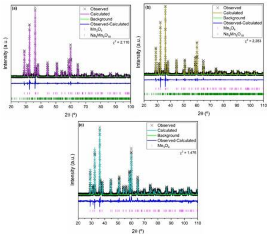
Figure 7: XRD patterns in the structure refinement of the samples (a) MnO 870 °C, (b) MnO 920 °C and (c) MnO 1150 °C.
