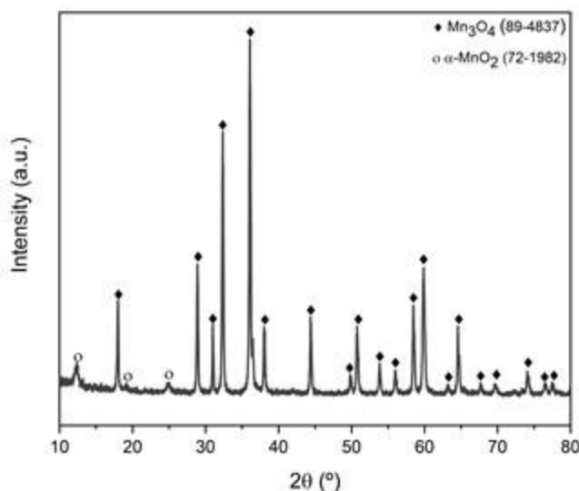
Figure 1: XRD patterns of the MnO sample synthesized via MAH. Assignments: ♦ = tetragonal \text{Mn}_3\text{O}_4 (JCPDS 89-4837) and ○ = tetragonal \alpha\text{-MnO}_2 (JCPDS 72-1982).
