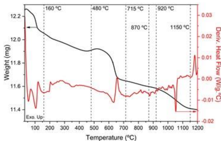
Figure 2: Thermal analysis of the MnO sample synthesized via MAH. The axes for weight change and for the derivative heat flow are indicated. The highlighted temperatures are those where the MnO sample was subsequently heat treated.
