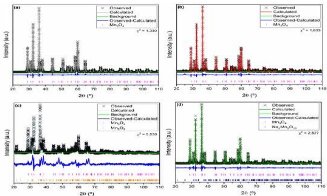
Figure 6: XRD patterns in the structure refinement of the samples (a) MnO, (b) MnO 160 °C, (c) MnO 480 °C and (d) MnO 715 °C.
