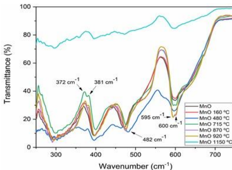
Figure 4: FTIR of MnO, MnO 160 °C, MnO 480 °C, MnO 715 °C, MnO 870 °C, MnO 920 °C and MnO 1150 °C samples.
