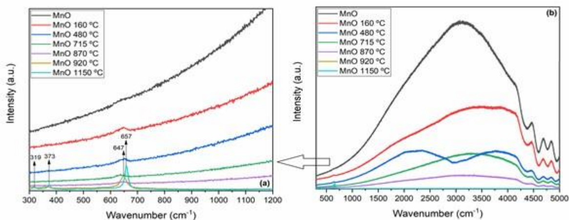
Figure 5: Raman scattering of MnO, MnO 160 °C, MnO 480 °C, MnO 715 °C, MnO 870 °C, MnO 920 °C e MnO 1150 °C samples. (a) 300-1200 cm -1 and (b) 300-5000 cm -1 .
