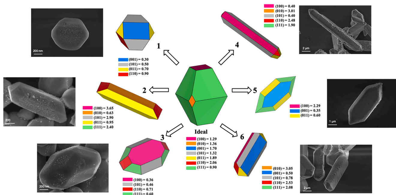
Fig. 4. Theoretical and experimental morphologies obtained by tuning the values of E_{surf} for Ag_2CrO_4 . The FE-SEM images for each sample is inserted for comparison purposes. Surface energy value in J/m^2 .
