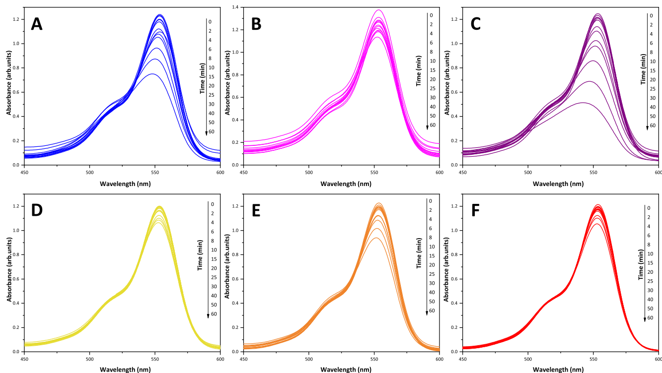
Fig. 7. UV-vis absorption spectra of the RhB aqueous solution in the presence of Ag_2CrO_4 powders, obtained by the CP method in water at A) 30, B) 60 and C) 90 °C and in ammonia at D) 30, E) 60 and F) 90 °C.
