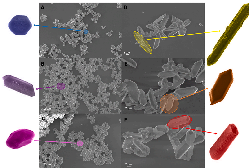
Fig. 1. FE-SEM images of \text{Ag}_2\text{CrO}_4 powders obtained by CP method in water at A) 30, B) 60 and C) 90 °C and in ammonia at D) 30, E) 60 and F) 90 °C.
