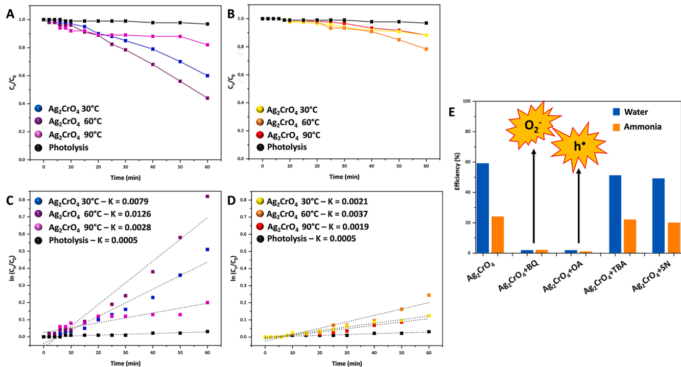
Fig. 8. A) Relative concentration of RhB dye ( C_t/C_0 ) versus time (min) of Ag_2CrO_4 powders obtained by CP method in water at different temperatures and B) in ammonia. (C) Reaction kinetics of RhB degradation \ln(C_t/C_0) versus t (min) for of Ag_2CrO_4 powders in water and D) in ammonia. E) Efficiency of degradation (%) of RhB dye under exposure to UV-vis radiation, in the presence of Ag_2CrO_4 and different scavengers for the both samples synthesized at 60 °C.
