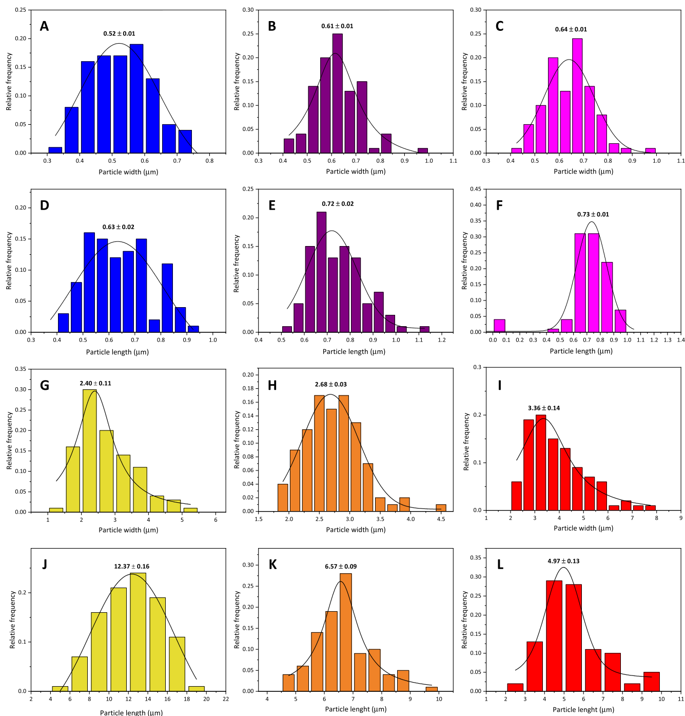
Fig. 2. Width and length distribution of \text{Ag}_2\text{CrO}_4 powders obtained by CP method in water at A-D) 30, B-E) 60 and C-F) 90 °C and in ammonia at G-J) 30, H-K) 60 and I-L) 90 °C.
