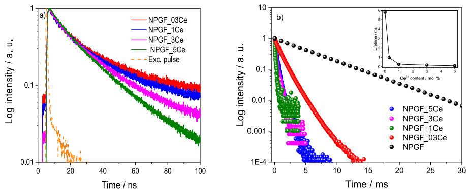
Fig. 5. Photoluminescence decay curves of \text{Ce}^{3+} doped and undoped NPGF glasses. (a) \text{Ce}^{3+}:5d \rightarrow 4f ( \lambda_{\text{exc}} = 289 nm \lambda_{\text{em}} = 350 nm) and (b) \text{Gd}^{3+}:^6\text{P}_j \rightarrow ^8\text{S}_{7/2} ( \lambda_{\text{exc}} = 273 nm \lambda_{\text{em}} = 311 nm).
