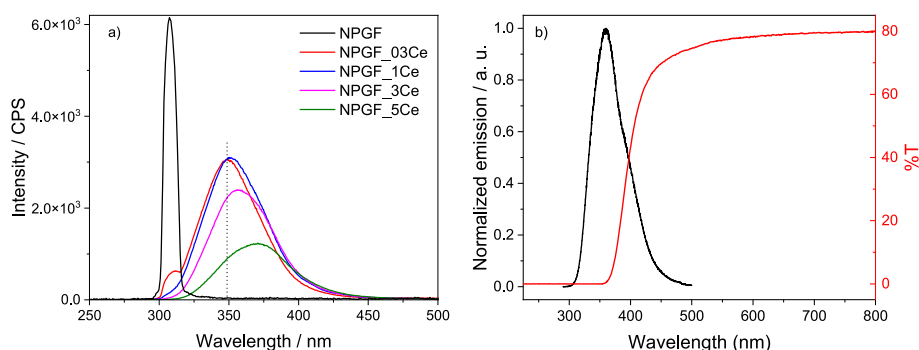
Fig. 6. (a) X-ray induced scintillation spectra of Ce 3+ doped and undoped NPGF glasses; (b) transmission and emission spectra of the representative NPGF_5Ce sample.
